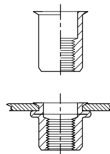
MR = glava z malim robom / reduced countersink head
