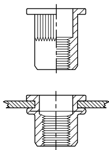
VR = glava z velikim robom / flat (cylindrical) head
