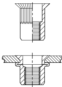
V = vgrezna glava / countersink head
